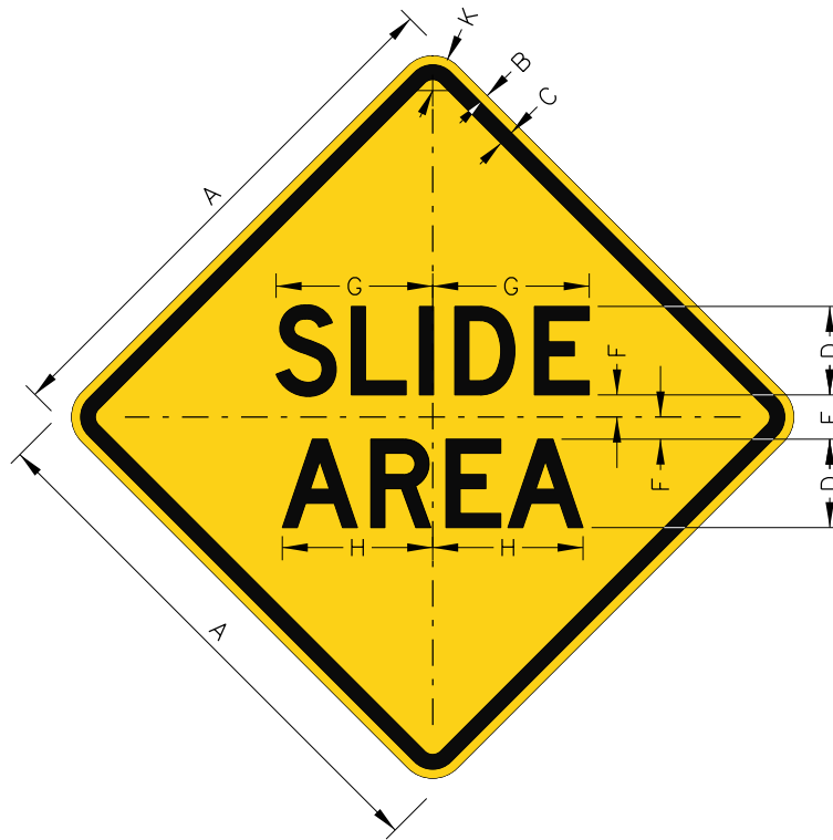
W8-1403 SLIDE AREA
