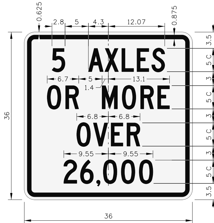
R2-201P TRUCK DEFINITION
