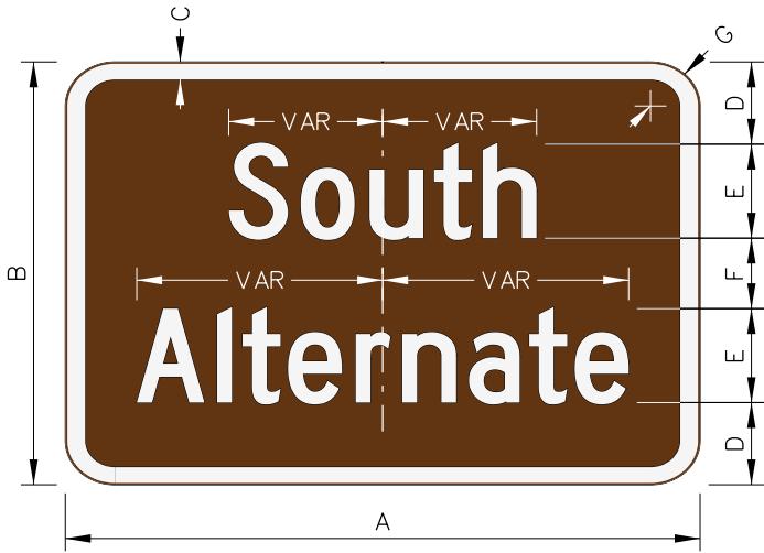
EXAMPLE AUTO TOUR PLAQUE
