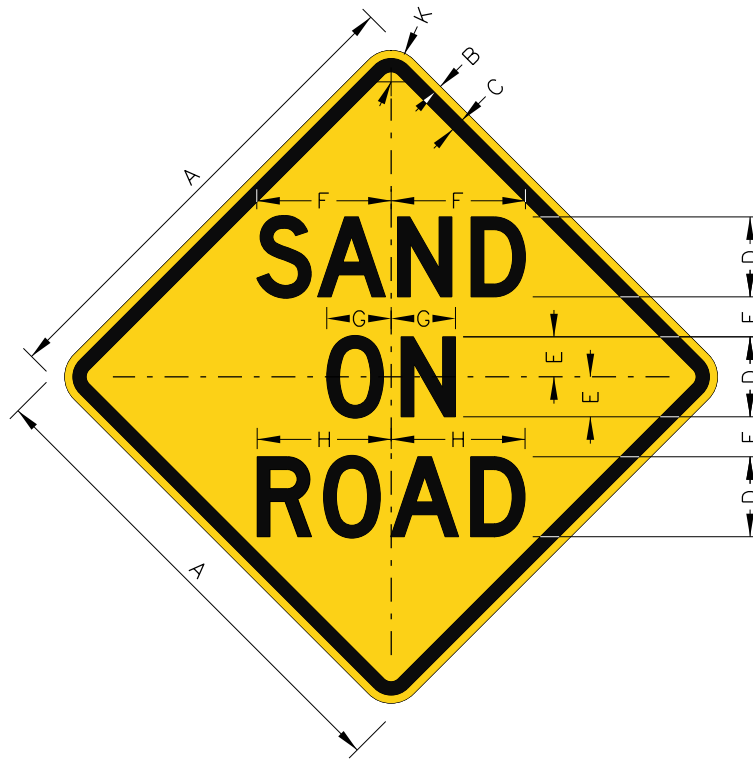
W8-701 SAND ON ROAD
