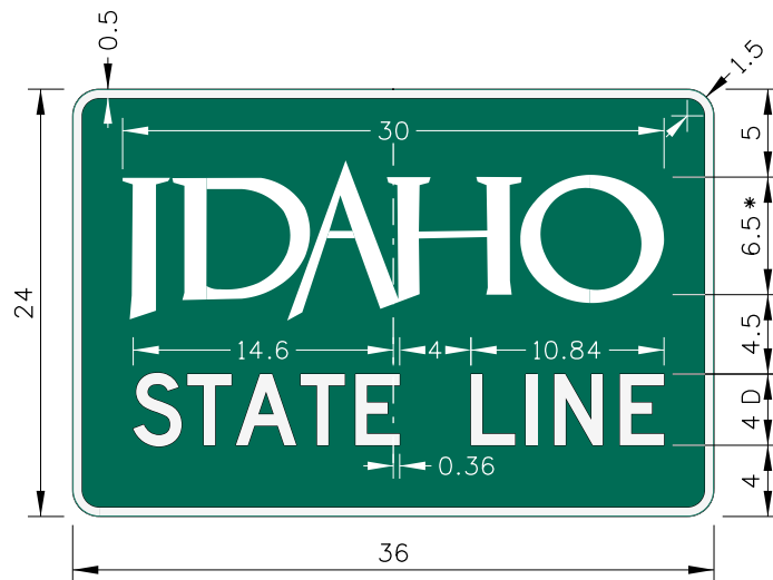
I-2 IDAHO STATE LINE
