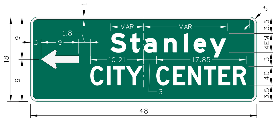
D1-101 BYPASSED COMMUNITY
