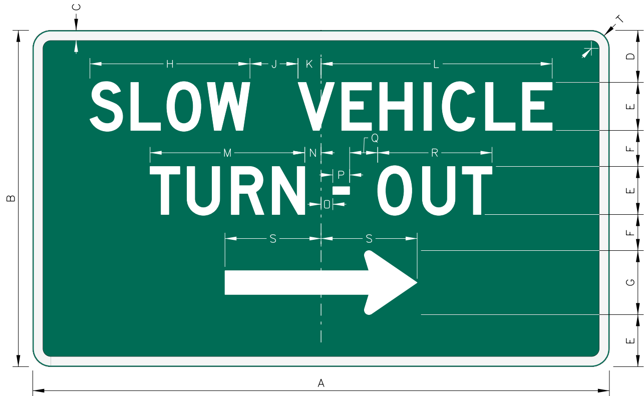
D17-701 SLOW VEHICLE TURN-OUT
