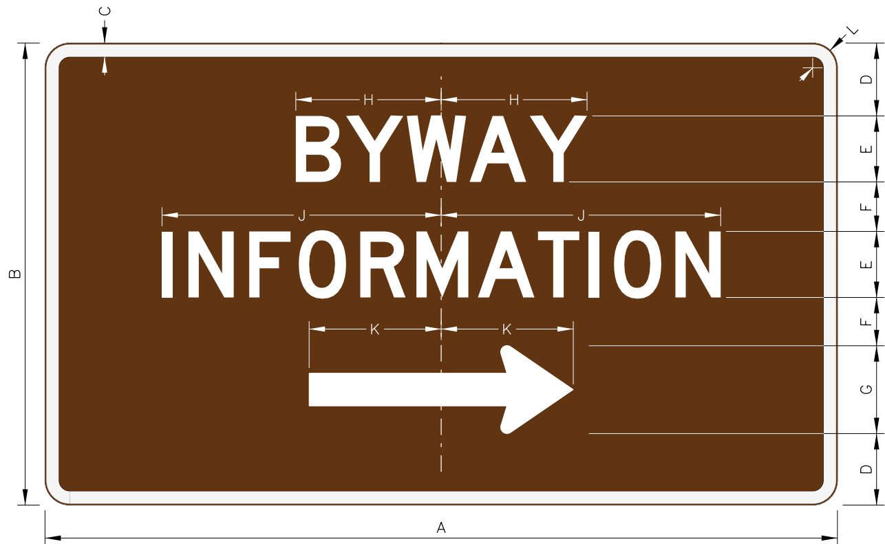
D5-2101 BYWAY INFORMATION
