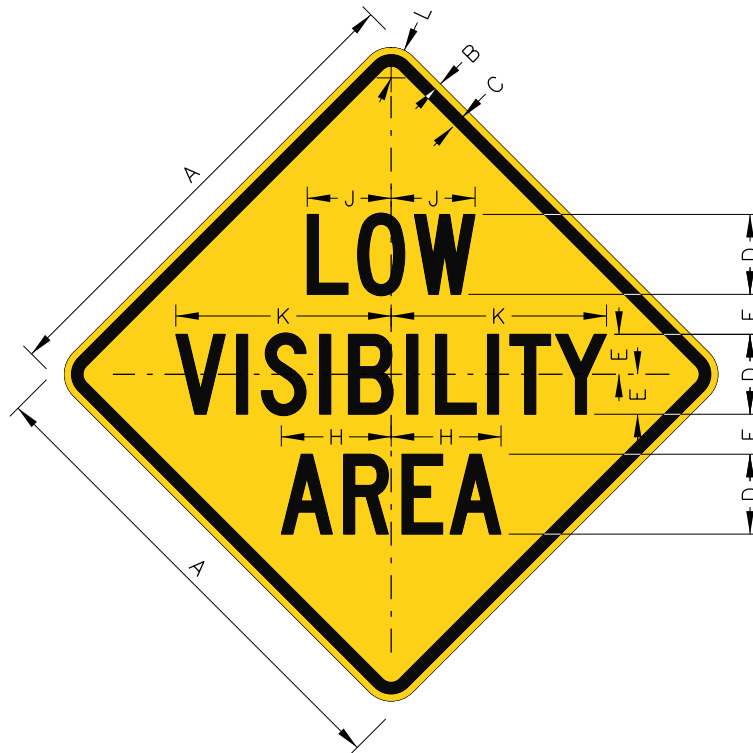
W8-2201 LOW VISIBILITY AREA
