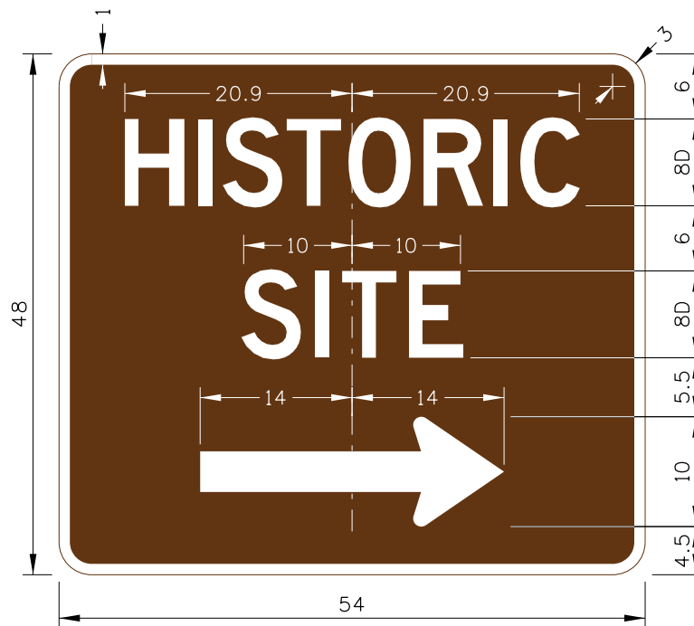
D5-2301 HISTORIC SITE
