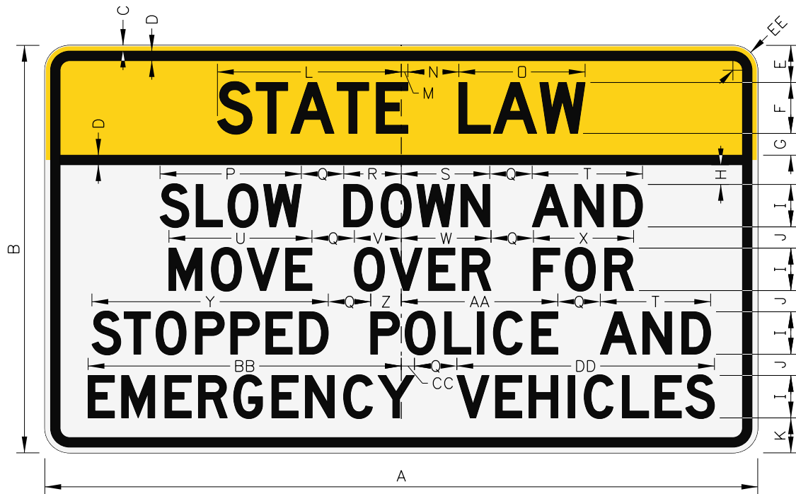
R16-101 SLOW DOWN AND MOVE OVER
