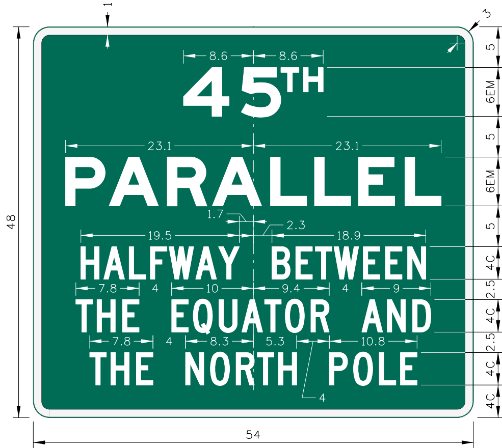
EXAMPLE I-3 MISCELLANEOUS INFORMATION
