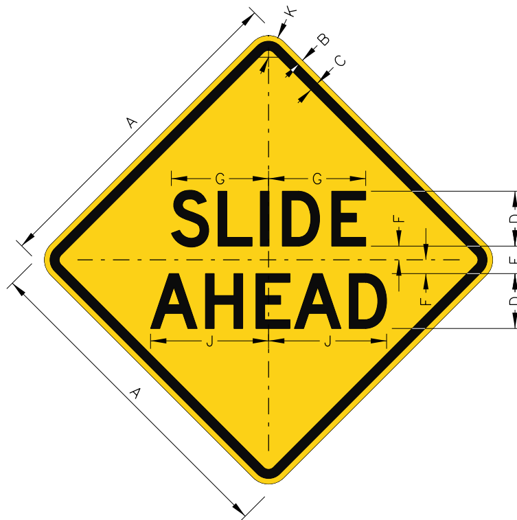
W8-1404 SLIDE AHEAD
