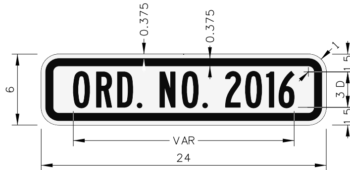
R2-501P ORDINANCE NUMBER PLAQUE
