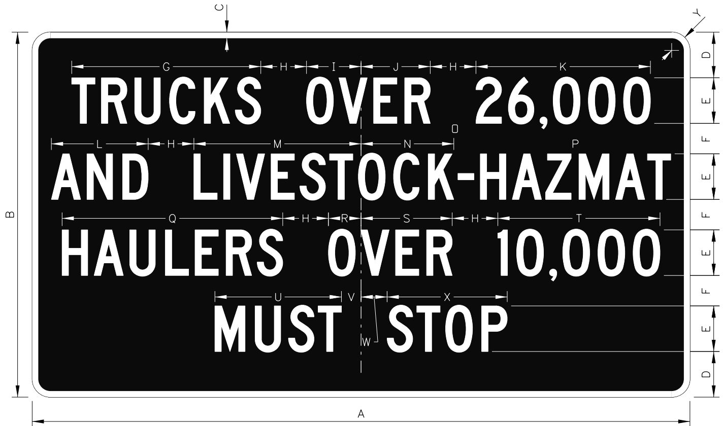
R13-101 WEIGH STATION
