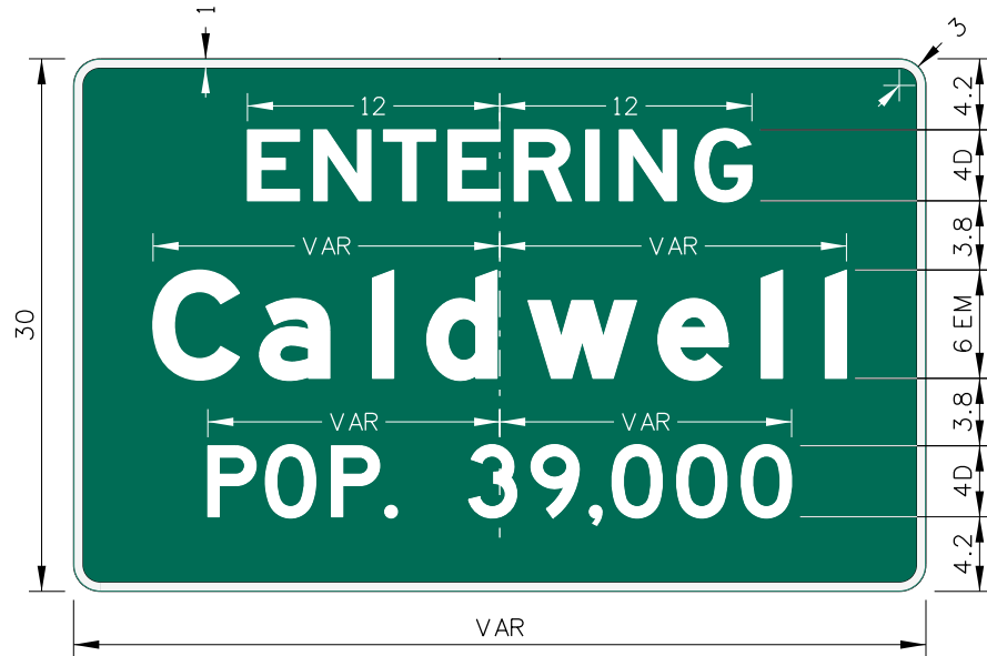
EXAMPLE I-2 JURISDICTIONAL BOUNDARY
