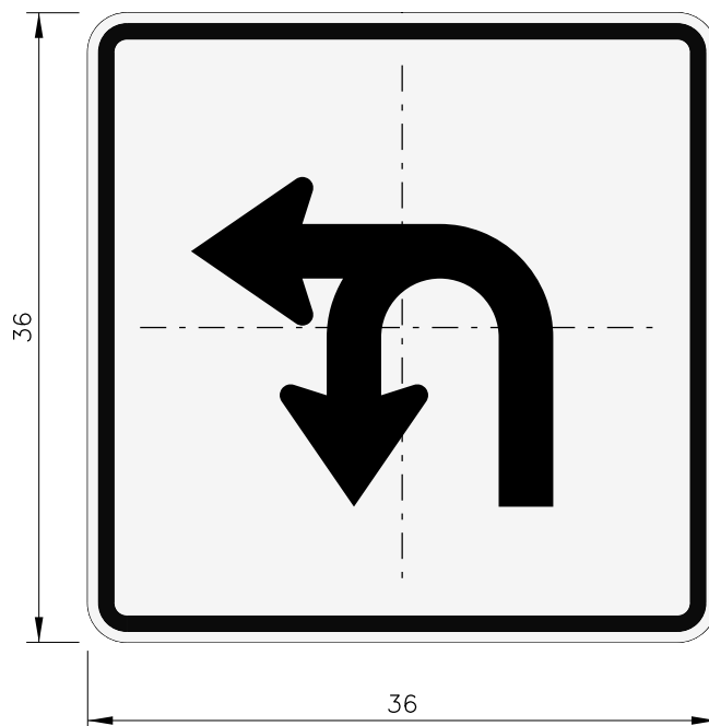
R3-6 ( Modified) OPTIONAL MOVEMENT LANE CONTROL
