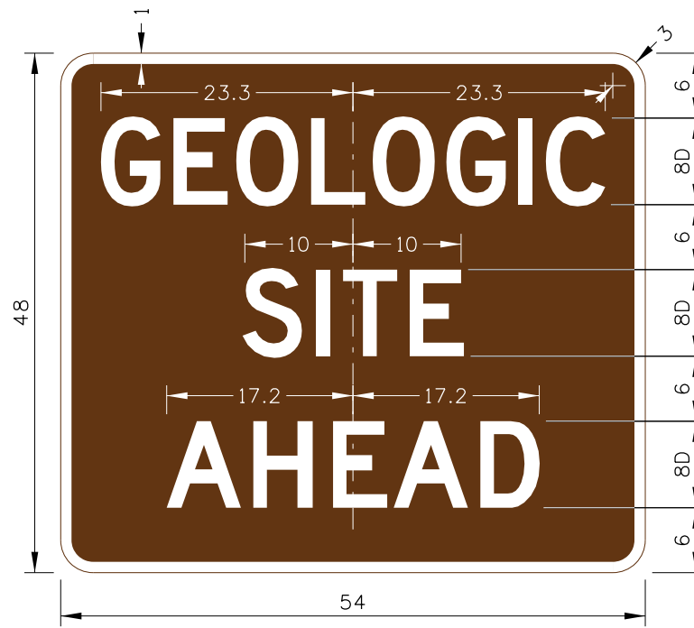
D5-2401 GEOLOGIC SITE AHEAD
