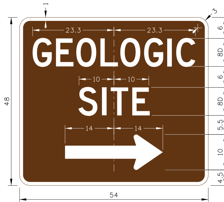
D5-2501 GEOLOGIC SITE
