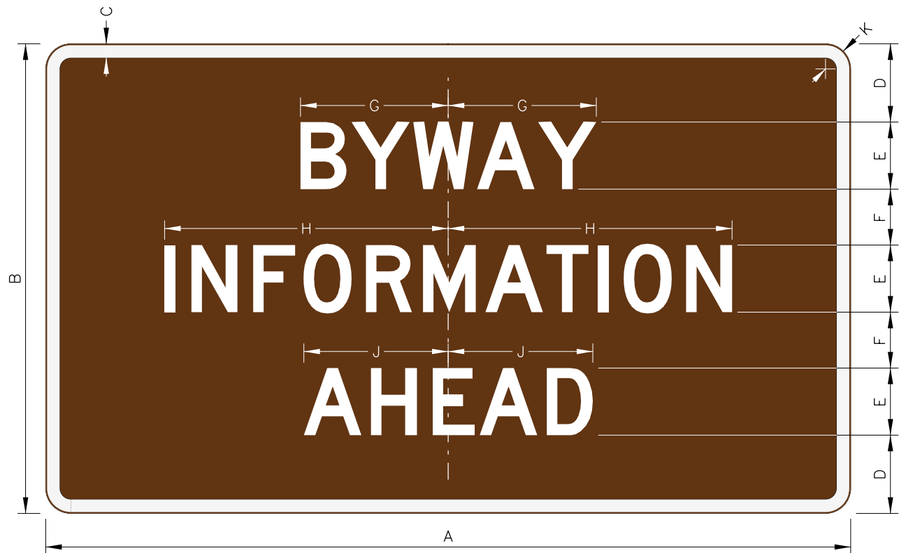
D5-2001 BYWAY INFORMATION AHEAD
