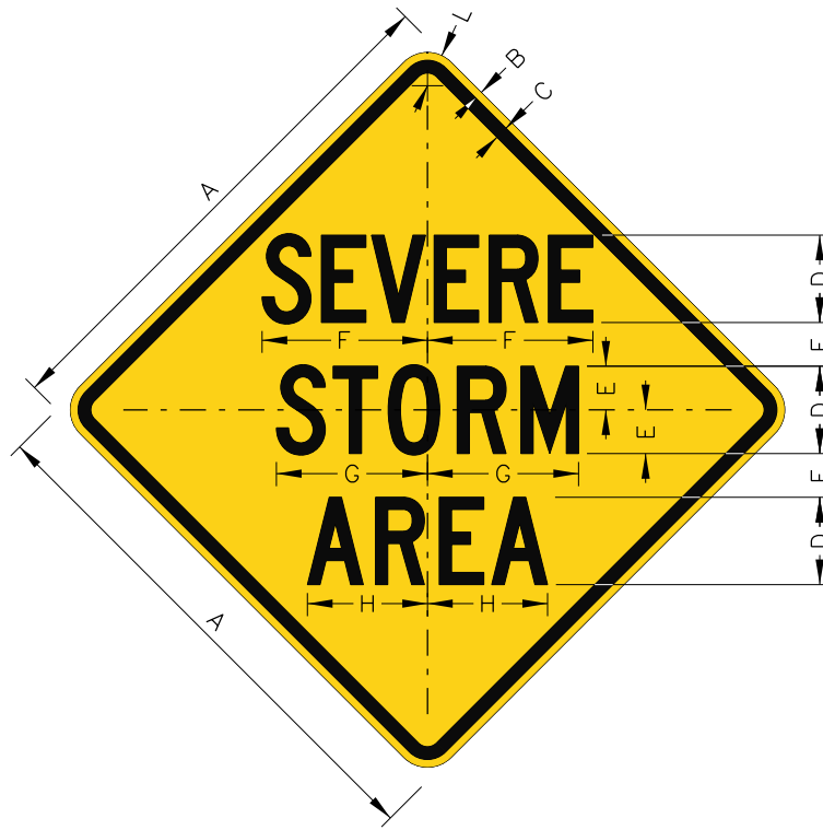
W8-2101 SEVERE STORM AREA
