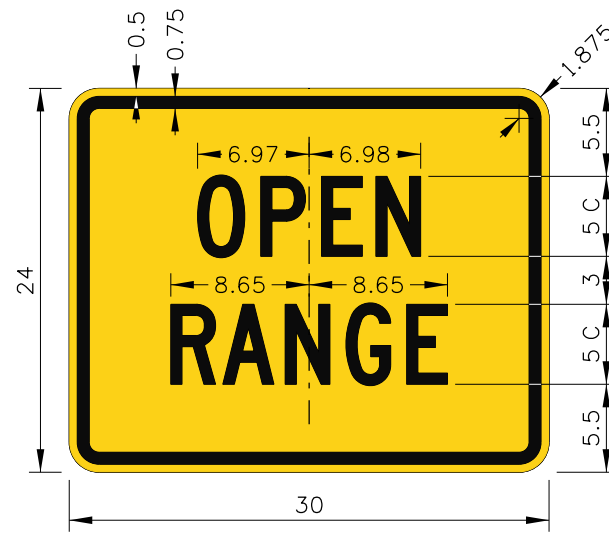
W16-901P OPEN RANGE PLAQUE
