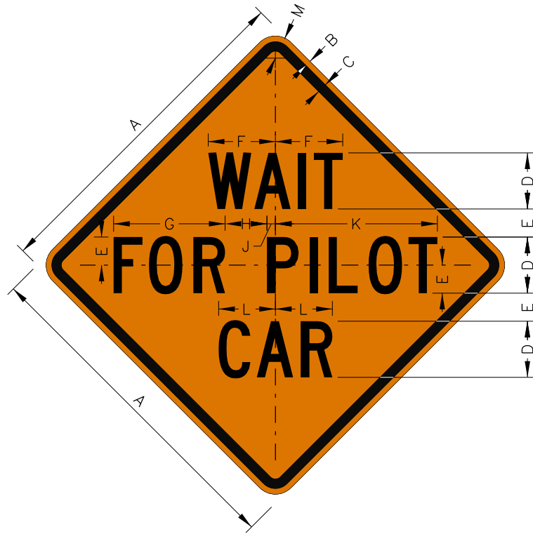
G20-401 WAIT FOR PILOT CAR
