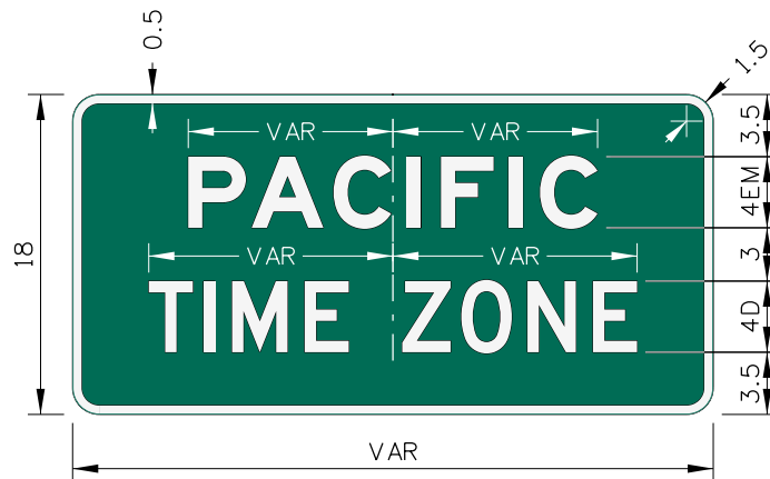
EXAMPLE I-3 MISCELLANEOUS INFORMATION
