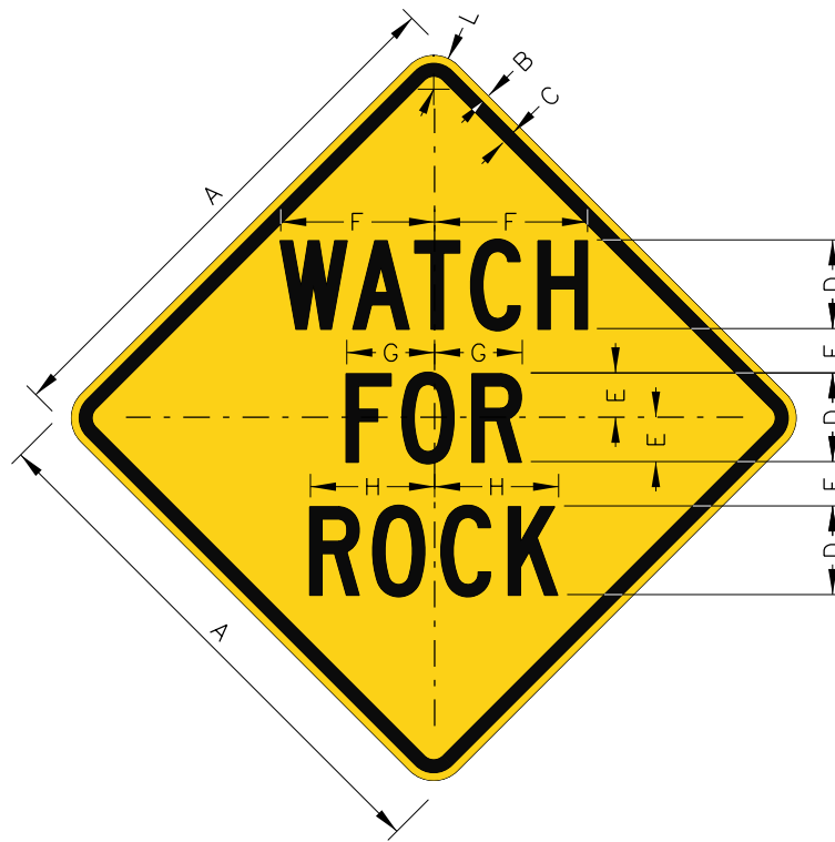
W8-1401 WATCH FOR ROCK
