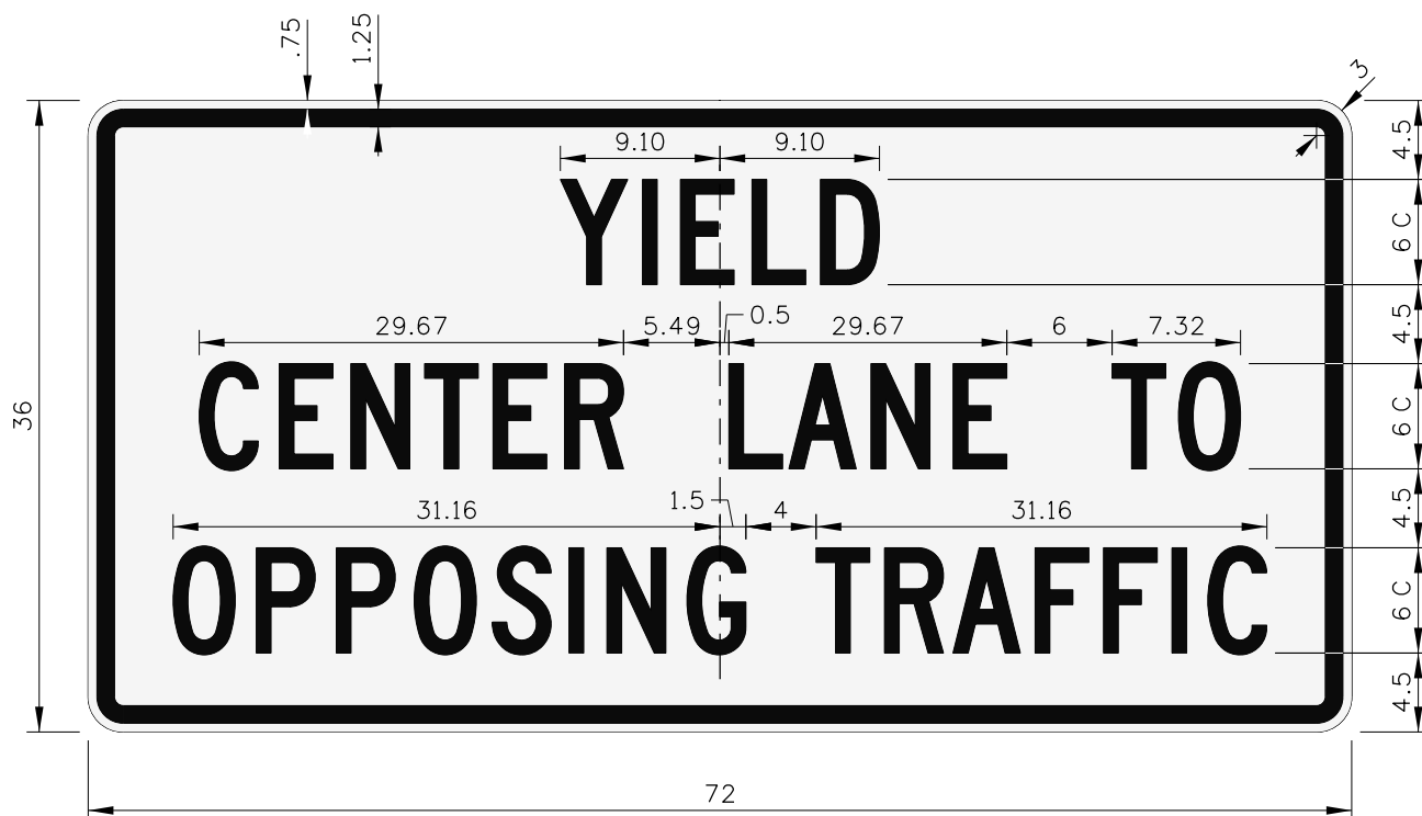
R4-101 YIELD CENTER LANE TO OPPOSING TRAFFIC
