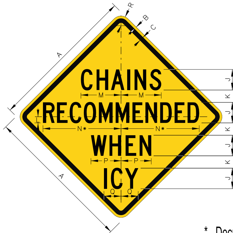
W8-1301 CHAINS RECOMMENDED
