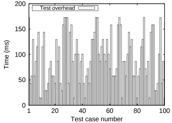
Figure 7: Performance of Test when |\gamma| = 10 .
