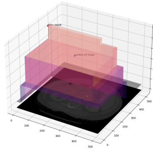
(b) 1 iteration
