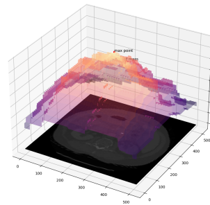
(c) 10 iterations
