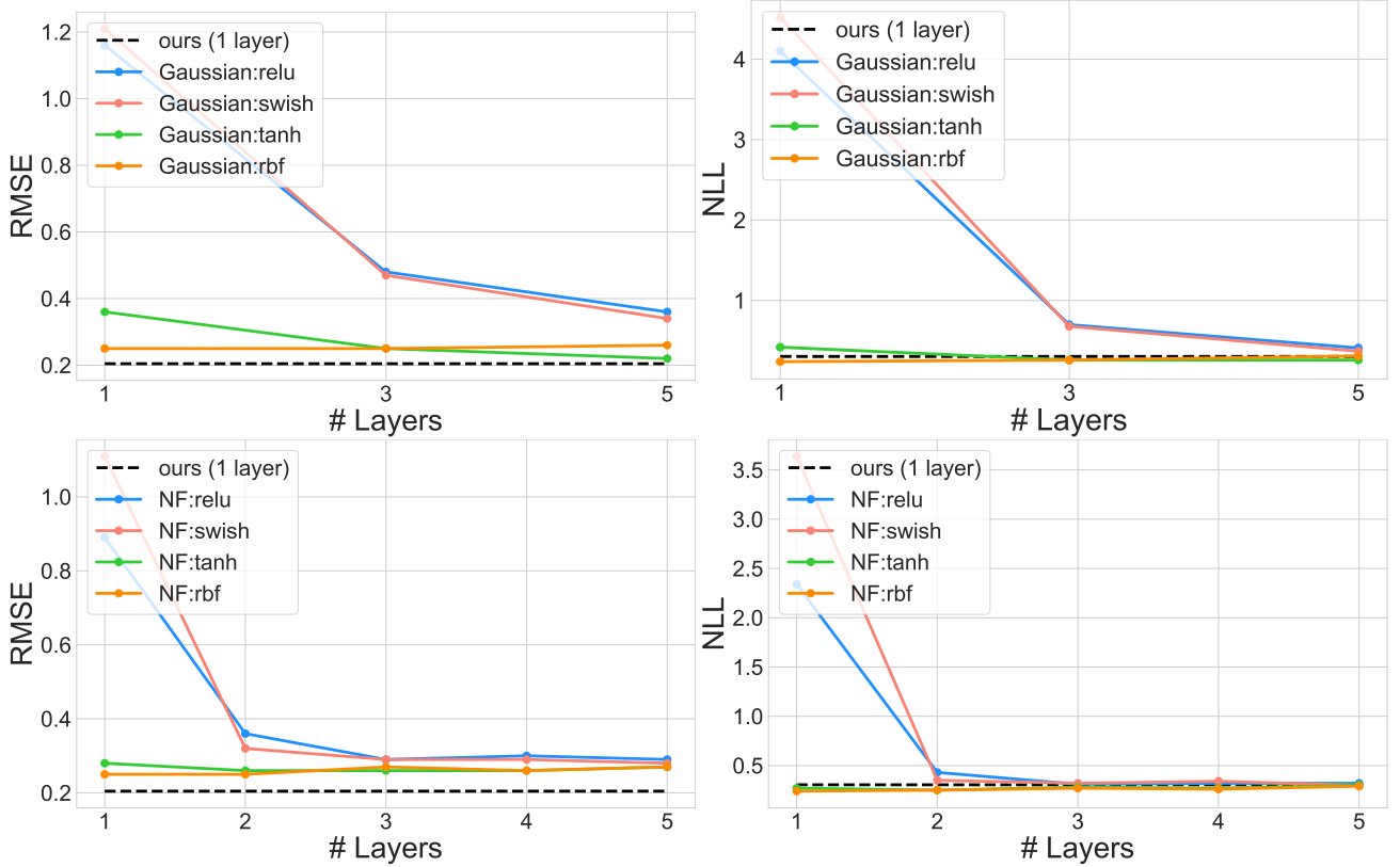
Figure 14: Comparison of different priors, activation functions and BNNS depth in Tran et al. [2022] method in terms of RMSE ( left column ) and NLL ( right column ) on test data. We observe that this method with Gaussian prior ( top row ) usually get better results with a larger number of hidden layers. Contrary, using Normalizing Flow prior get better results only for some ( worse ) activations. The largest increase of quality might be observed for the worst activation functions. We find that our approach ( dashed black line ) has better, or similar results in terms of both NLL and RMSE.
