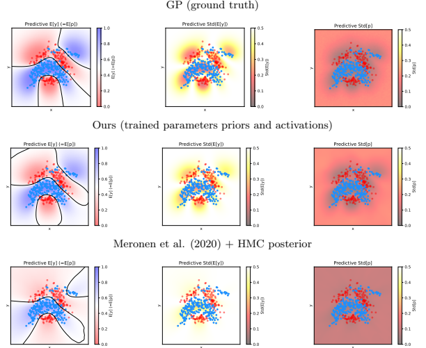
Figure 5: Posterior predictive distributions for a BNN with trained parameter priors and activations (ours; 2nd row) and for a BNN with analytically derived activations (3rd row). The first column illustrates class probabilities, the second column shows the total variance in class predictions, and the last column depicts the epistemic uncertainty component of the total uncertainty. Here, we show posteriors obtained using HMC, while in Sec. D.4 of the Appendix, we provide an extended version of the figure that includes results obtained using the original code from Meronen et al. [2020] (which uses MC-Dropout instead of MCMC), along with additional numerical results.
