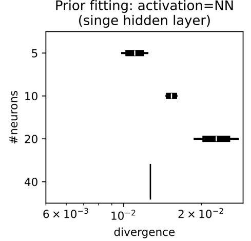
Figure 10: Prior matching quality: fixed depth.
