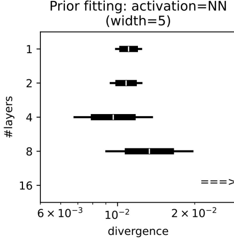
Figure 9: Prior matching quality: fixed width.
