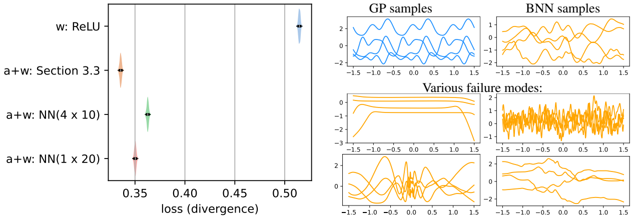
Figure 11: Quality of matching BNNs to the prior of a GP with the Periodic kernel ( \ell = 1, p = 1 ). (Left): Evaluation of models with trained parameter priors (denoted by w ) and with trained both weights priors and activations (denoted by a+w ). (Right): Samples from the ground truth GP, a well-fitted BNN and BNN outliers with poor final loss. As explained in Sec. 3.7, or because of the insufficient modeling capacity of \phi , gradient-based optimization may fail to capture a GP functional prior.
