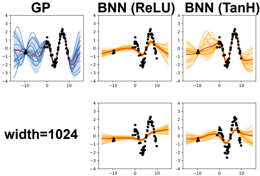
Figure 13: Comparison of Normalizing Flow prior with a one-layer BNN having a varying number of neurons and ReLU ( middle column ) or TanH ( 3rd column ) activation function. We provide a BNN with a narrow hidden layer (50 neurons) as the baseline and compare it against a BNN with a wider hidden layer (1024 neurons). We observe that even wider hidden layer does not provide a better GP approximation due to the lack of theoretical guarantees when using non-Gaussian priors.
