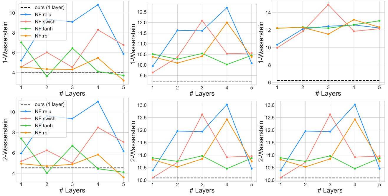
Figure 19: Comparison of Tran et al. [2022] method with a Normalizing Flow prior and different number of hidden layers. In this plot, we present \mathcal{W}_1^1 (top row) and \mathcal{W}_2^2 (bottom row) for the regions R3 , R4 ∪ R2 , and R1 ∪ R5 from left to right side. The appropriate regions might be found in Fig. 16.
