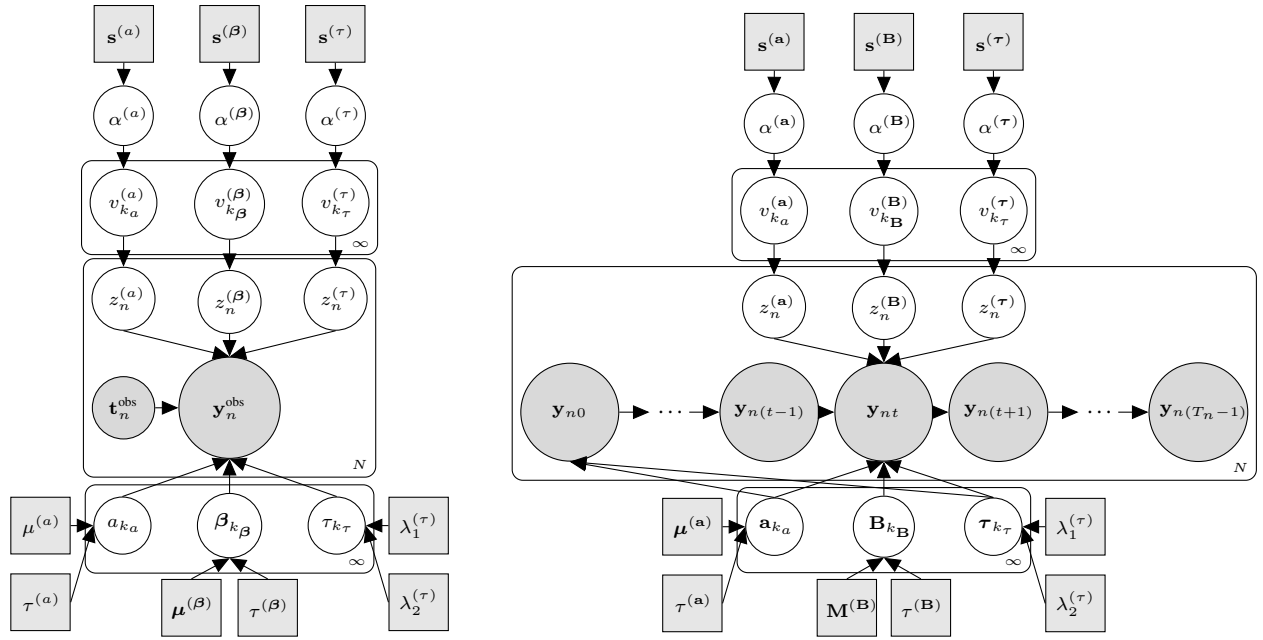
Figure 2: Plate diagram of MMM with left ) nonlinear growth model and right ) multivariate autoregressive model.
