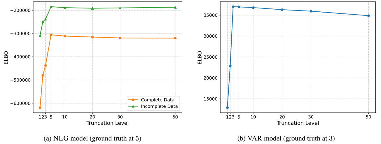
Figure A.2: The ELBO vs. different truncation levels for simulations. Both models achieve their highest ELBO when the truncation level matches the ground truth number of clusters.
