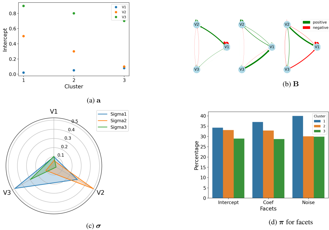
Figure A.5: Parameter estimations of the VAR model on the simulated dataset when truncation level is 10. The true number of clusters for all three facets is 3.
