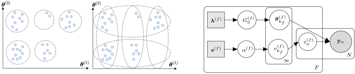
Figure 1: left ) single-facet versus multi-facet clustering. right ) nonparametric Bayesian multi-facet mixture model
