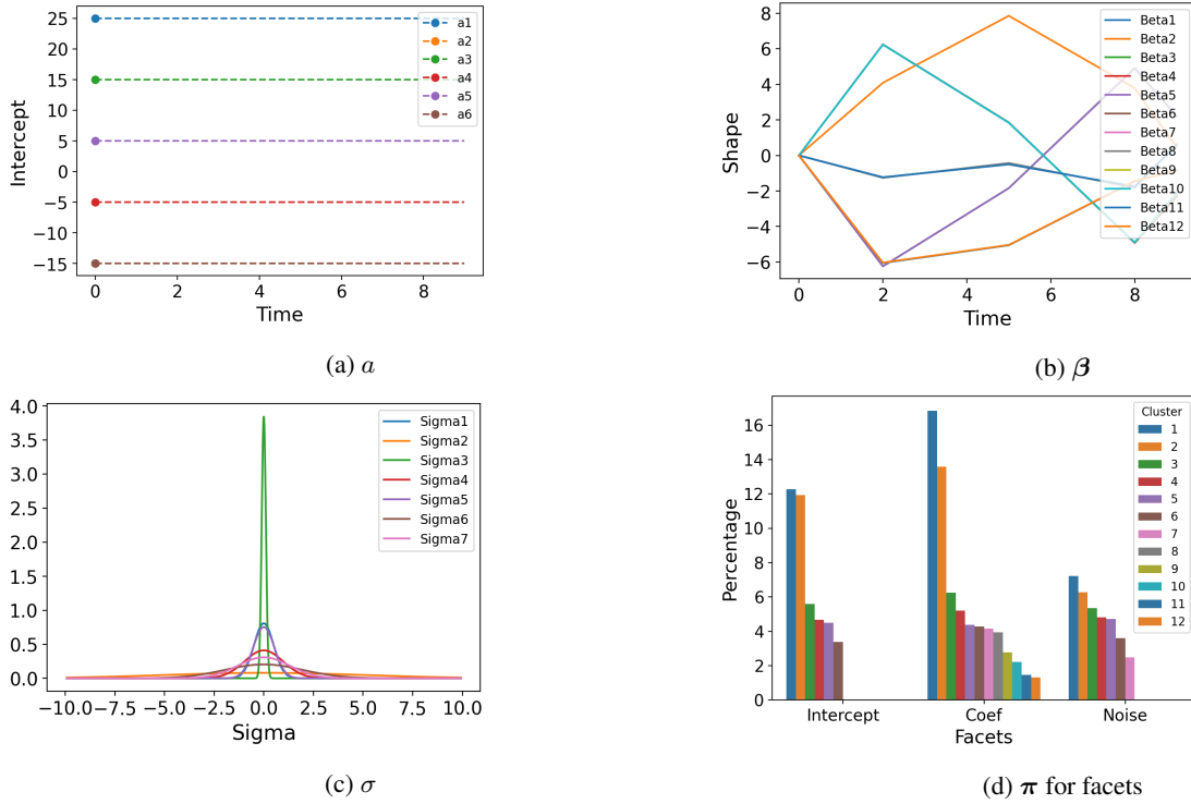
Figure A.4: Parameter estimations of the NLG model on the large incomplete dataset at truncation level 50.
