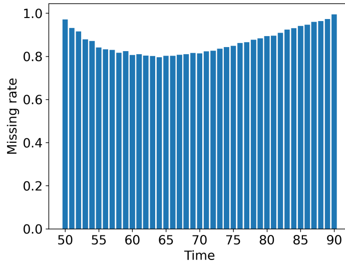
Figure A.7: The missing rate of ELSA data for the NLG model at each age time point.
