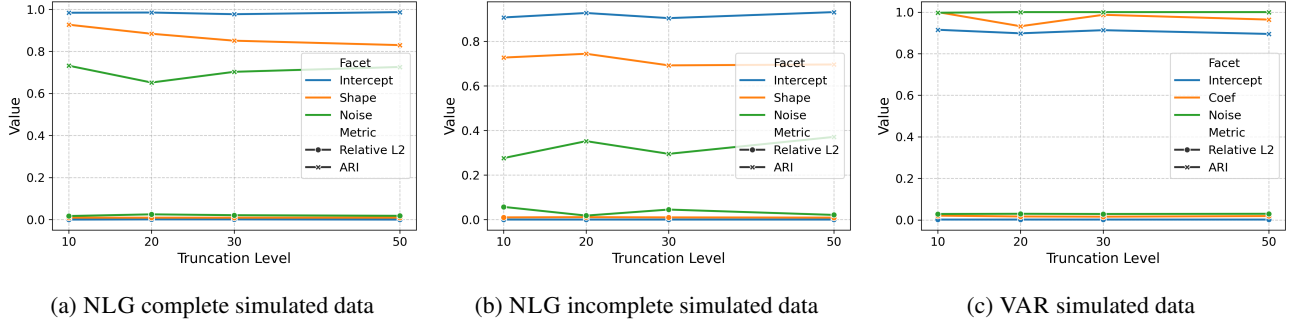
Figure A.1: The relative L_2 errors and ARI vs. different truncation levels for simulations.
