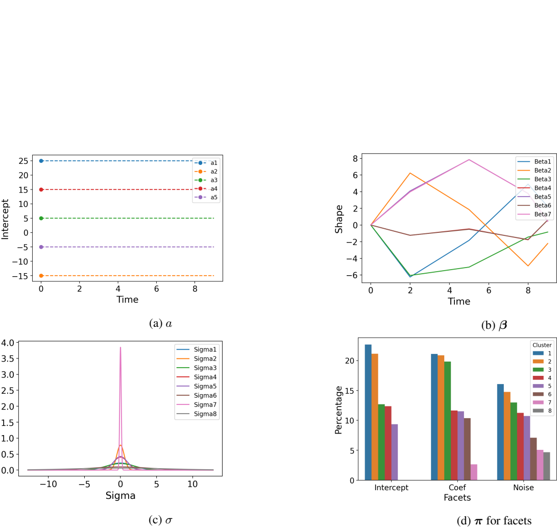
Figure A.3: Parameter estimations of the NLG model on the large incomplete dataset at truncation level 10. The true number of clusters for all three facets is 5.
