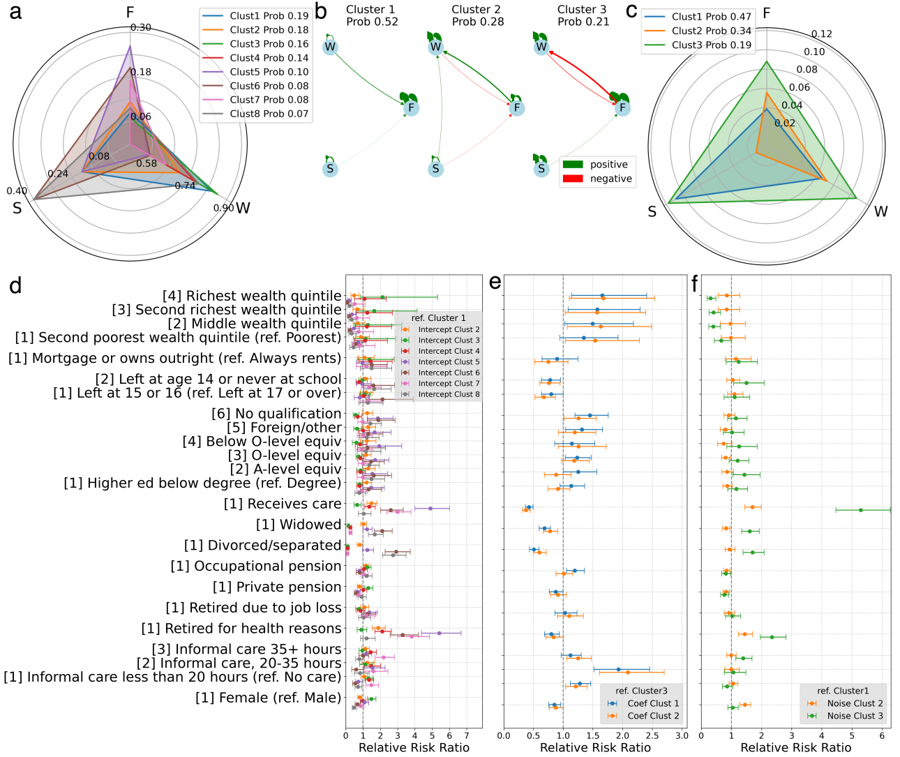
Figure 5: a) Eight intercept clusters. b) Three coefficient matrix clusters. c) Three noise clusters. Relative risk ratios (RRRs) for d) intercept e) coefficients and f) noise clusters.
