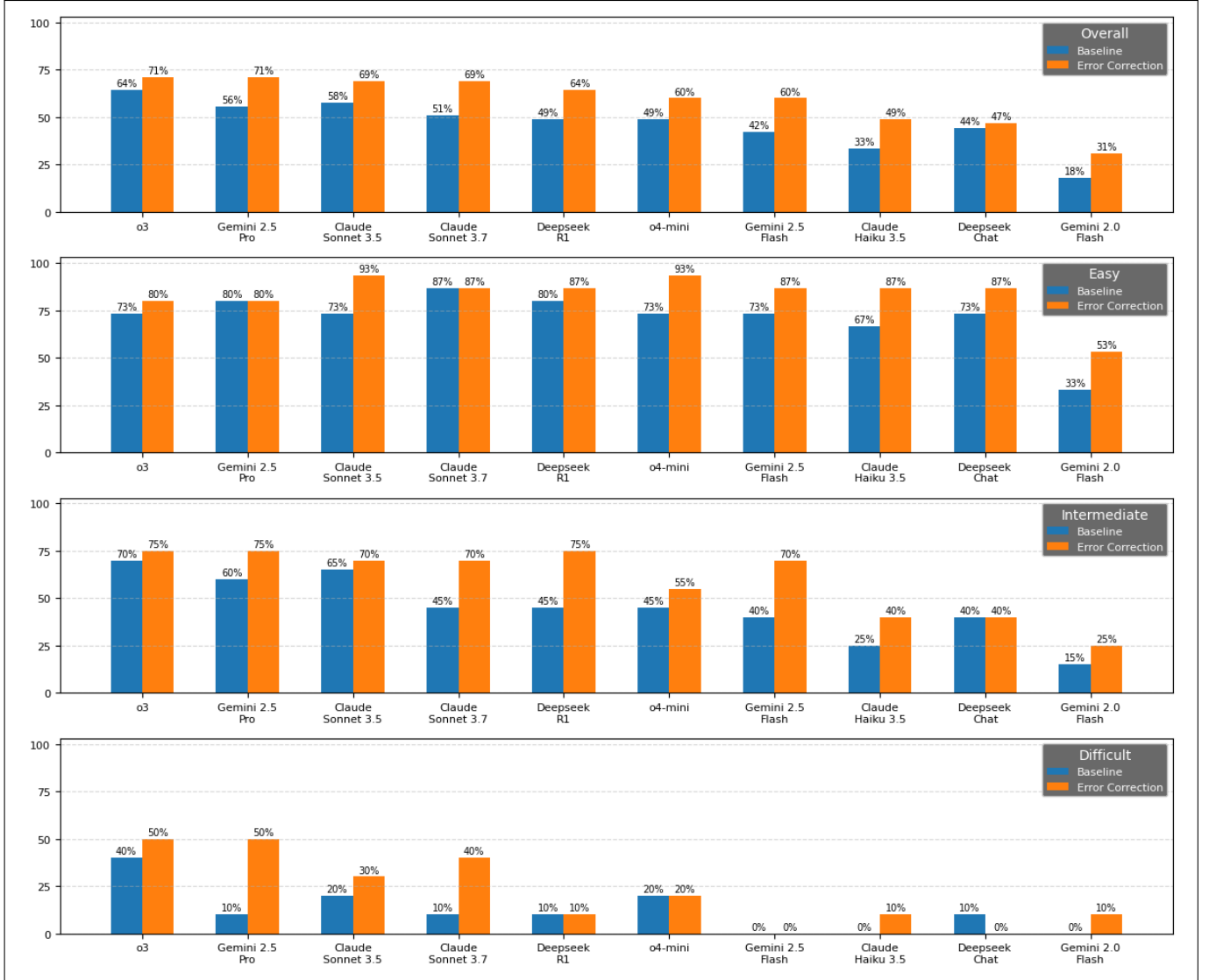
Figure 2: Baseline vs Error Correction, grouped by difficulty.
