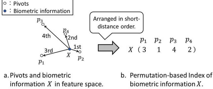
Fig. 4. A scheme for creating a permutation-based index from a template and pivots.
