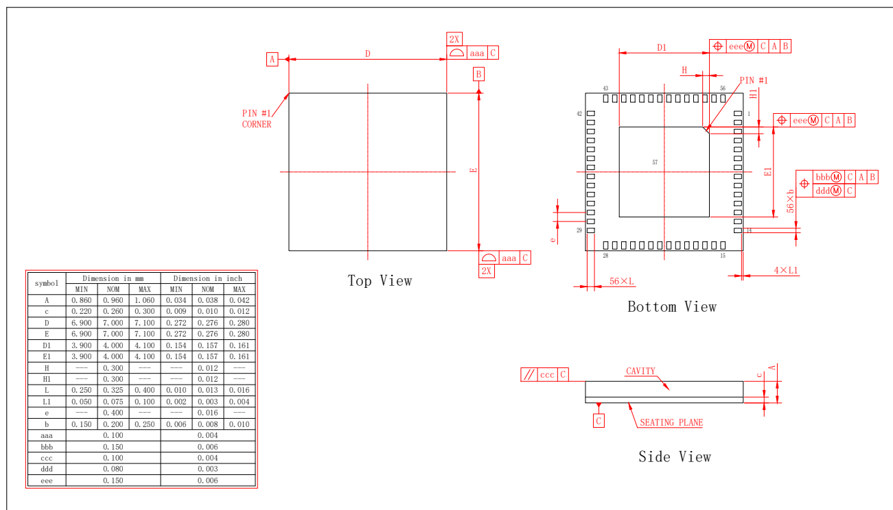
Figure 6-1. LGA56 (7×7 mm) Package
