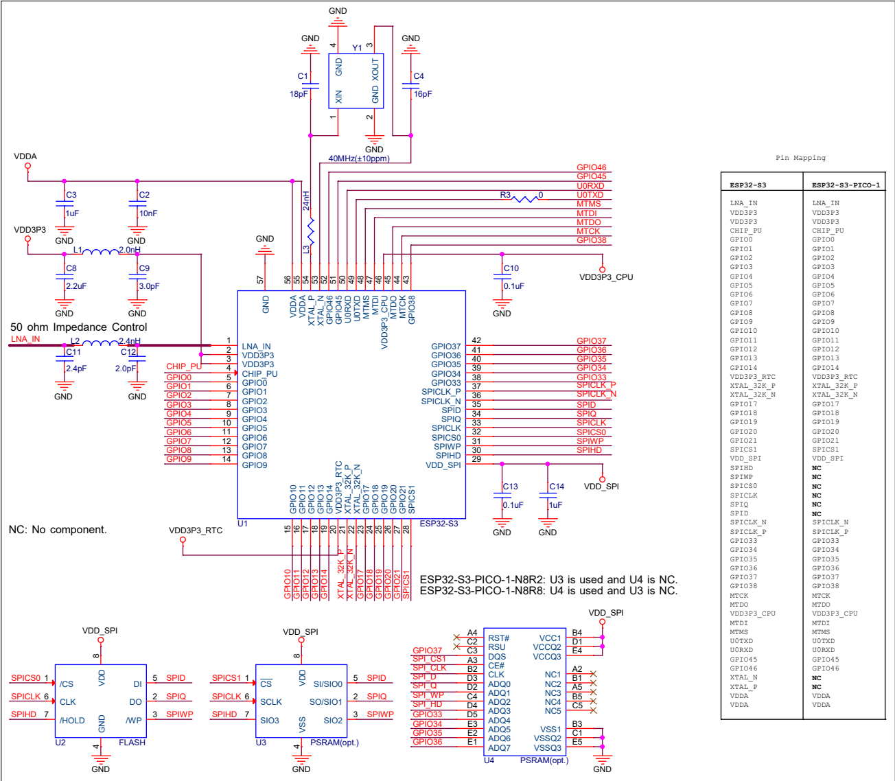
Figure 4-1. ESP32-S3-PICO-1 Schematics
