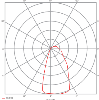
Ambient Optic 4000K
