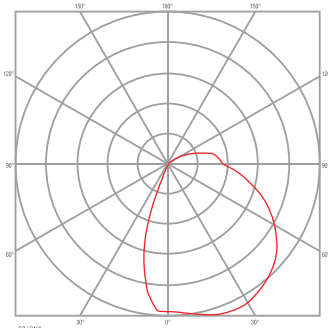
Cove Glow Optic 4000K
