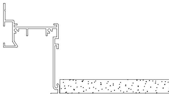
Flange Trim Gypsum/Millwork/Other Material
