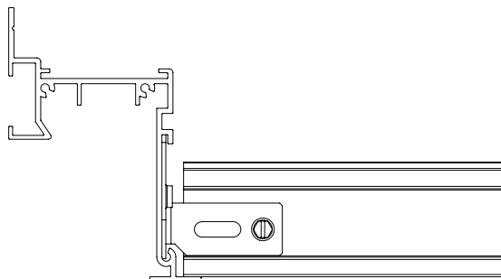
9/16" Dimensional Grid (Bolt Slot or Bull Nose)
