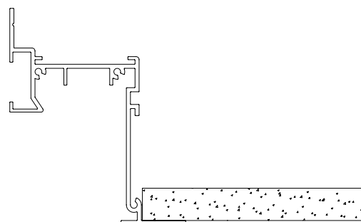
Mud Flange Gypsum
