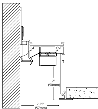
Flange Trim Gypsum/Millwork/Other Material
