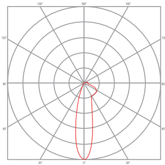
Graze Optic 4000K
