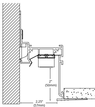
Mud Flange Gypsum
