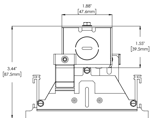
15/16" GEMINI Single Lens GEM4-XX-X-X-24-XX-X-W-UNV
