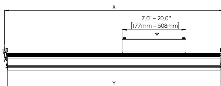
9/16" GEMINI Single Lens GEM4-XX-X-X-15/15B-XX-X-W-UNV
