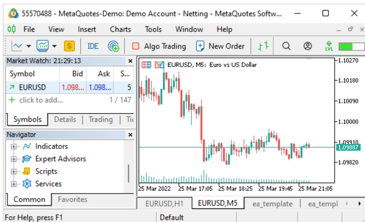
MetaTrader 5
